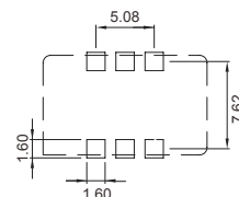
Top View Suggested Layout
